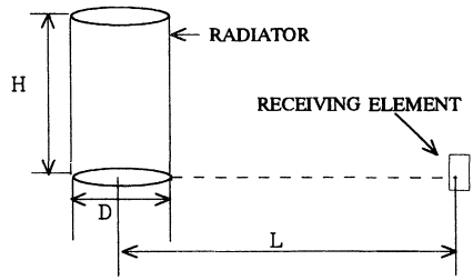
FIGURE 3 Cylindrical model of flame radiation 8,9)
