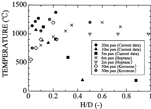
FIGURE 13 Relationship between the maximum temperature along with flame axis and dimensionless height from initial liquid surface
