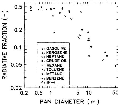
FIGURE 2 Relationship between radiative fraction and pan diameter for various fuels fires 5)
