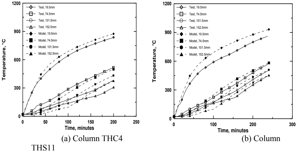
Figure 2 Comparison of temperature distribution at various depths for HPC columns
