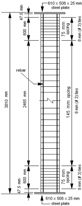
(a) Elevation
