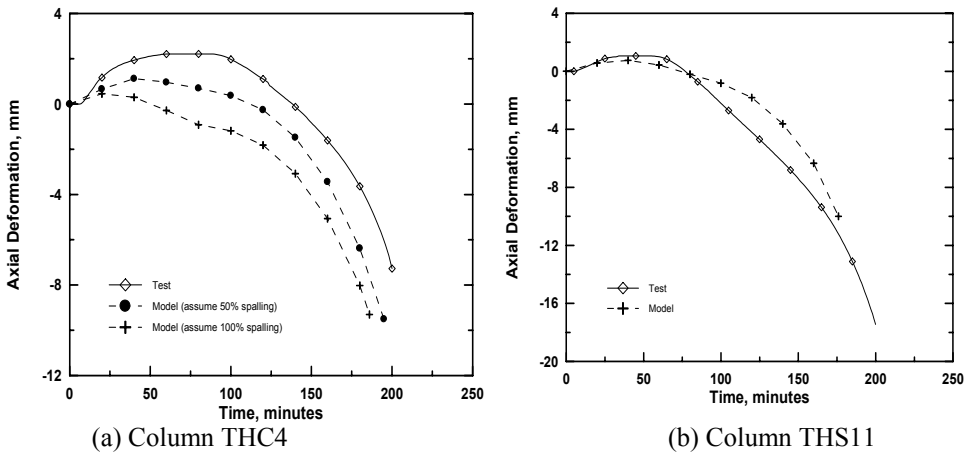
Figure 3 Comparison of axial deformation for HPC columns
