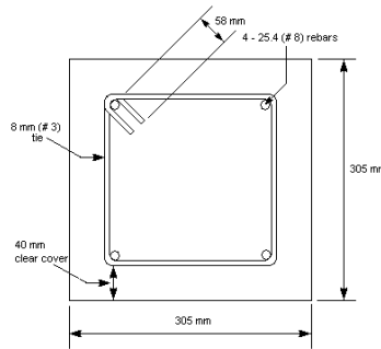
(b) Cross section
