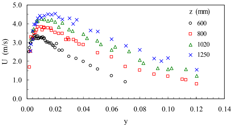
Figure 9. LDV measurements of vertical velocity, U , vs. normal distance, y , for different heights, z , from the leading edge at a mass transfer rate, \dot{m}'' = 5.4 \text{ g/m}^2 \text{ s} . during the summer of 1982. The measurements were not correlated at the time. The
